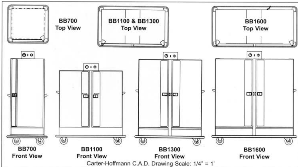
Carter-Hoffmann C.A.D. Drawing Scale: 1/4" = 1'
